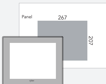
Panel cut
