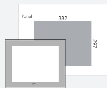
Panel cut
